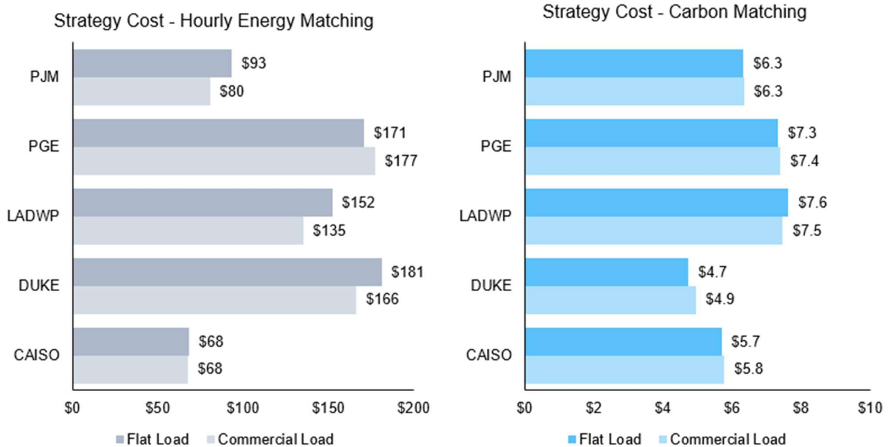
Figure 8: Cost comparison for the hourly energy matching and carbon matching strategies for customers with commercial load and flat load in each balancing authority
