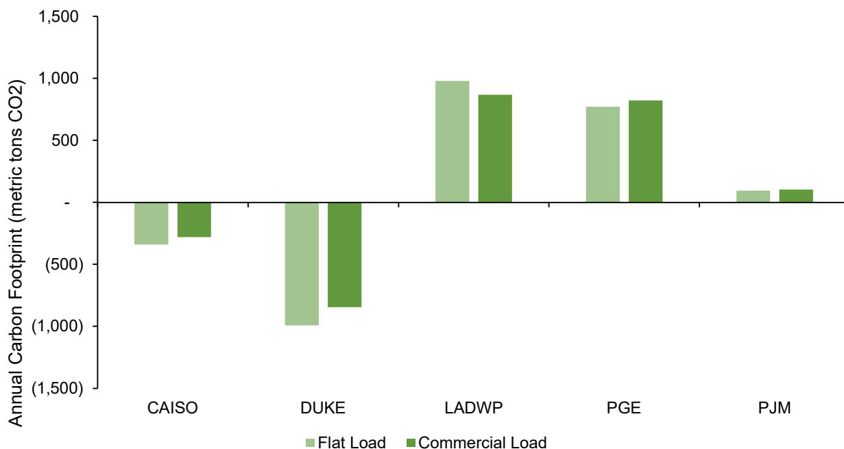
Figure 13: Comparison of carbon footprint for the annual energy matching strategy between the commercial load customer and the flat load customer. The commercial load footprint has been scaled up so that each customer uses the same amount of energy per year.
