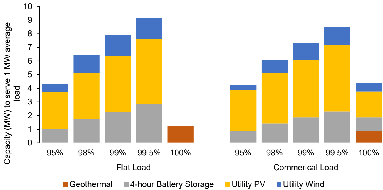
Figure 19: Capacity mix procured by customers with commercial load and flat load in CAISO, by CFE score. The commercial load customer’s capacity mix has been normalized to the same total load (8760 MWh / year) as the flat load customer.
