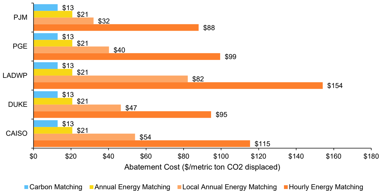
Figure 11: CO 2 abatement cost by strategy for customers with commercial load in each balancing authority. For hourly energy matching the target CFE score is 100%.
