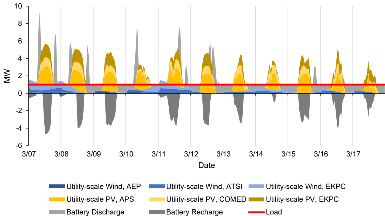
Figure 18: 10-day period in 2025 for customer in PJM balancing authority, 100% CFE, flat load
