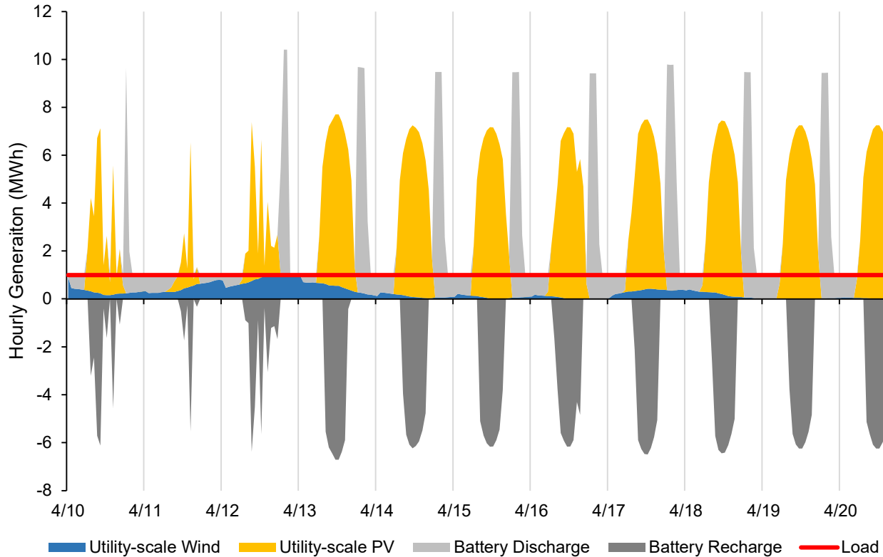
Figure 16: 10-day period in 2025 for customer in LADWP balancing authority, 100% CFE score, flat load
