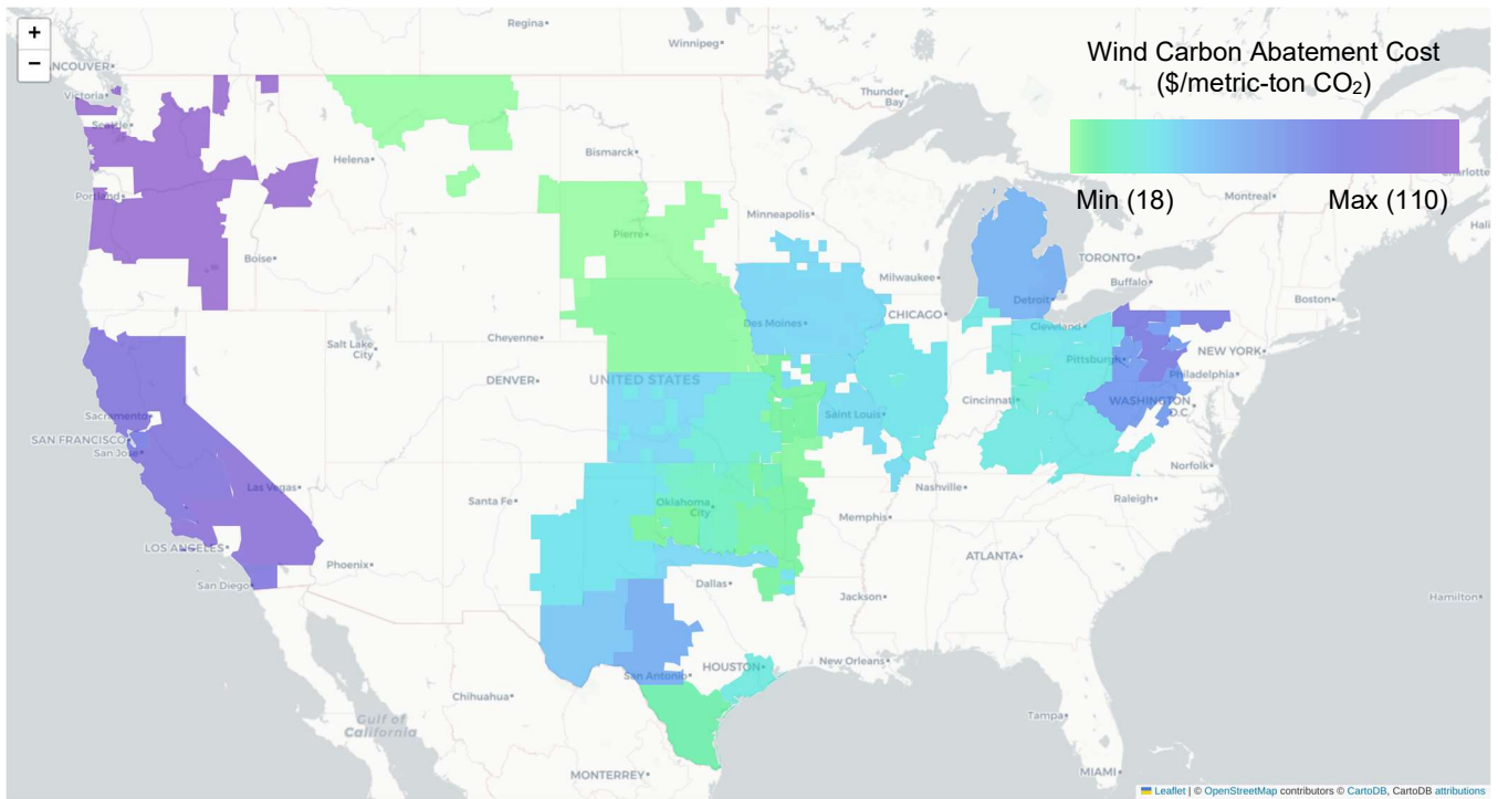
Figure 6: Carbon abatement cost for wind projects
